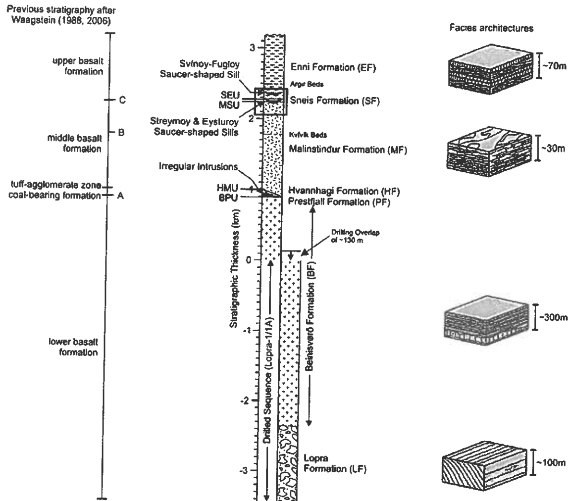
Figure 2. Stratigraphic subdivision of the FIBG. The previous subdivision is given to the left of the column for comparison. The facies architectures of the main formations are given to the right of the figure. The Lopra Formation is composed predominantly of hyaloclastites. The Beinísverð Formation is dominated by laterally extensive, basaltic simple sheet lobes. Conversely, the Malinstindur Formation is composed of compound basalt lava flows and the Enni Formation is composed of a mixture of these two facies architectures. The stratigraphic position of the Tunnel region at the boundary between Malinstindur, through Sneis, and Enni Formations is highlighted (red box).
