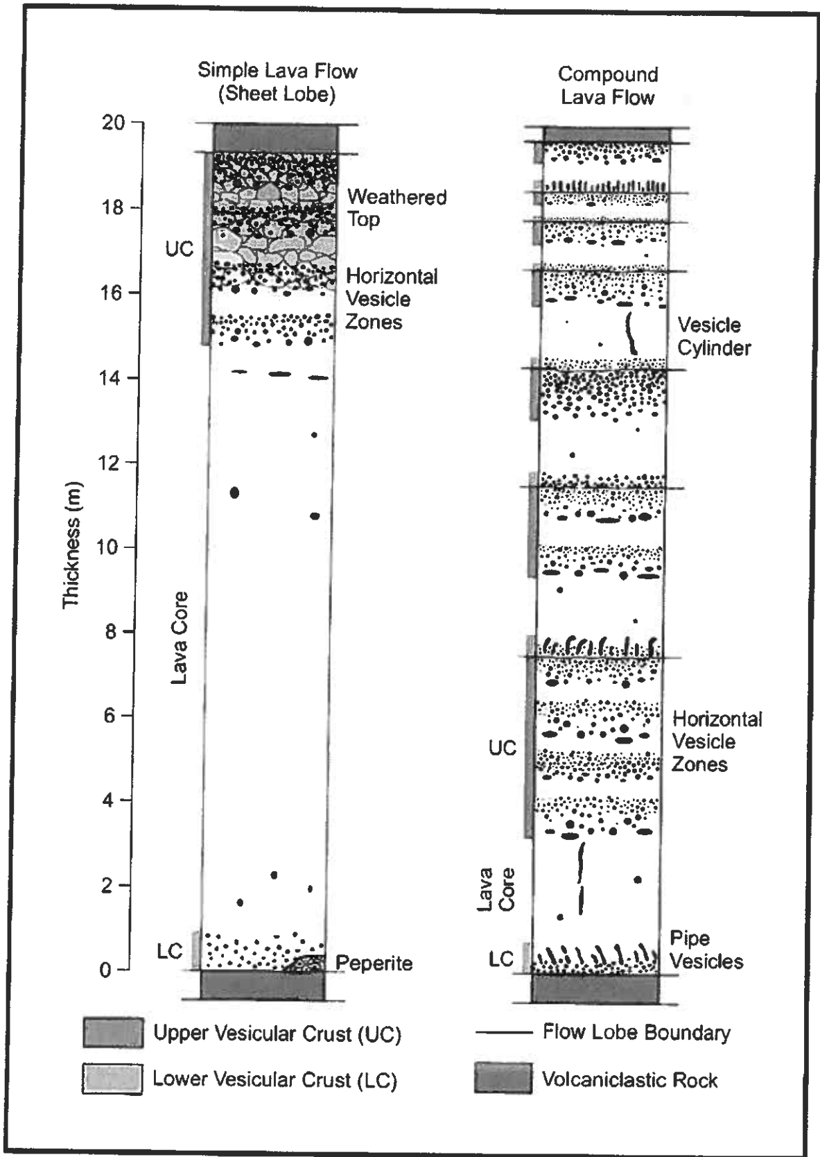
Figure 3. Idealized vertical profiles through a simple and a compound basalt lava flow.
