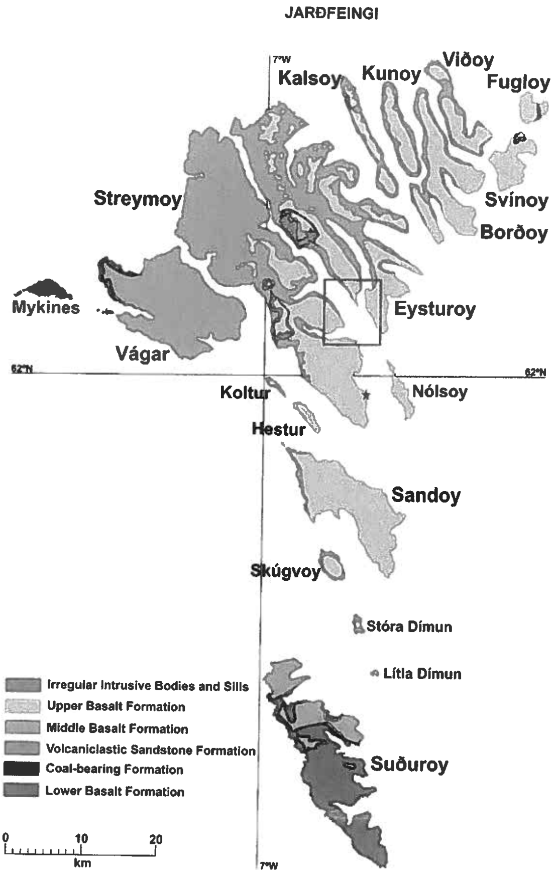
Figure 1. Geological map of the Faroe Islands. The Tunnel area is highlighted with a red box, and the location of the Glyvursnes-1 well (see text) is indicated with a red star. See also Fig. 2 for the formation characteristics and terminology.
