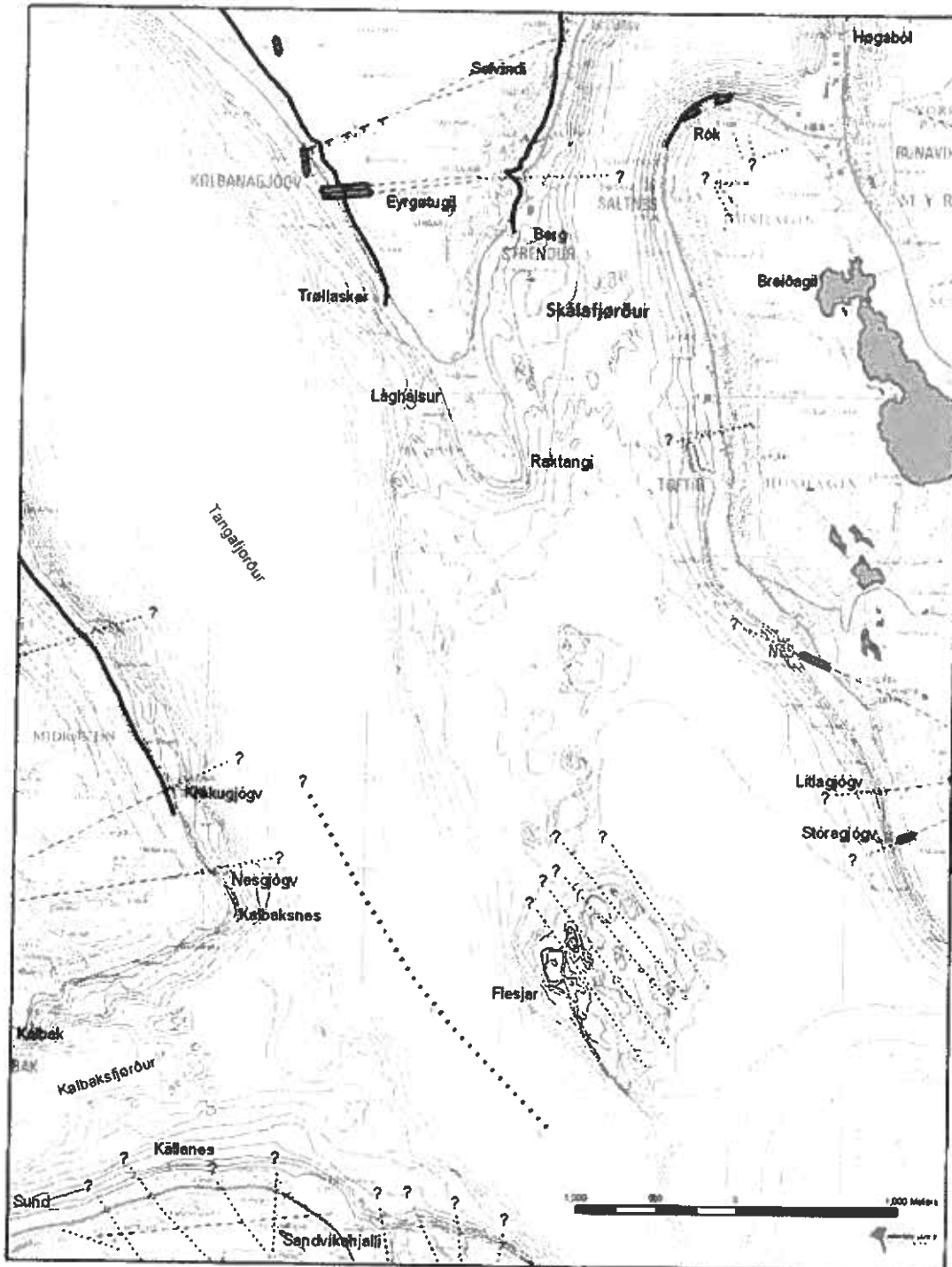
Figure 5. Map showing some main geological features, height and depth contours and place names. The solid black line indicates the approximate location of the Sneis Formation, with the underlying Malinstindur Formation (green colour) and overlying Enni Formation (paler colour). Stippled black lines indicate observed fracture zones while the dotted lines indicate other signs of potential fracture zones. Red signature indicates basaltic dykes. Be aware of the depth contour configuration in the Tangafjørður and Flesjar region showing a system of SE-NW orientated ridges and basins which may indicate the occurrence of systematic fracturing of the subsoil in this region. The tunnel is planned to extend from Sund on Streymoy to the regions near Selvindi and Breiðagil on each side of Skálafjørður, respectively, via a sub-sea roundabout.
